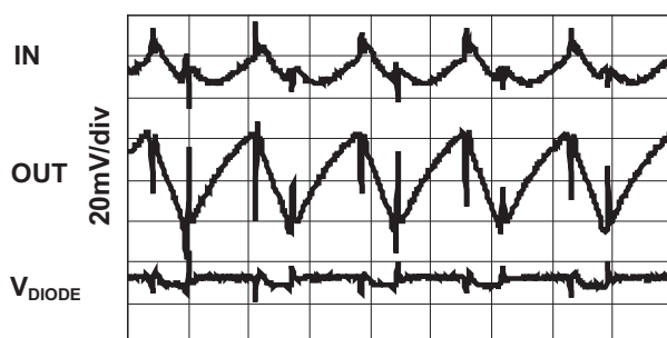
80mA Load Characteristics
