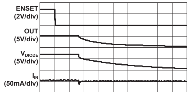
Turn-Off
