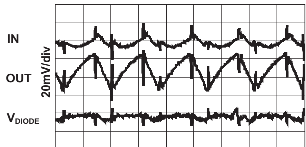
60mA Load Characteristics
