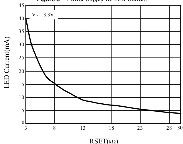
Figure 5 R SET vs. LED Current
