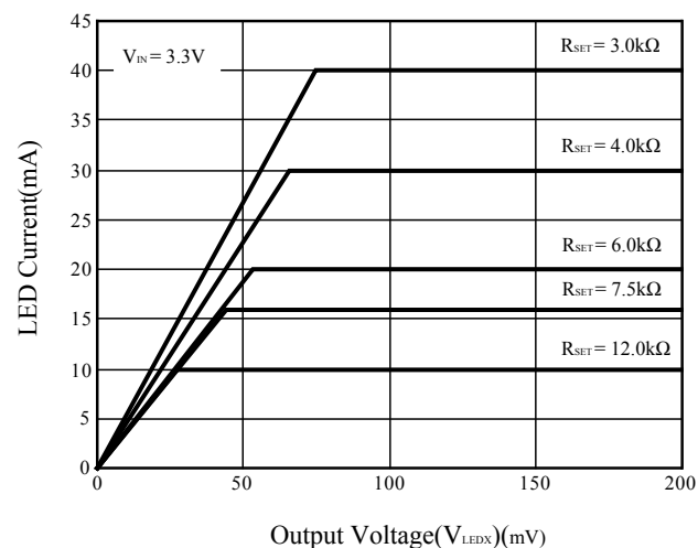
Figure 2 Output Voltage vs. LED Current
