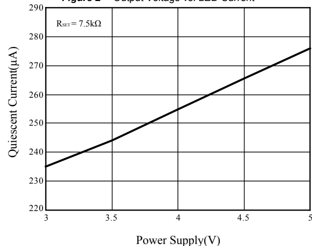
Figure 4 Power Supply vs. Quiescent Current
