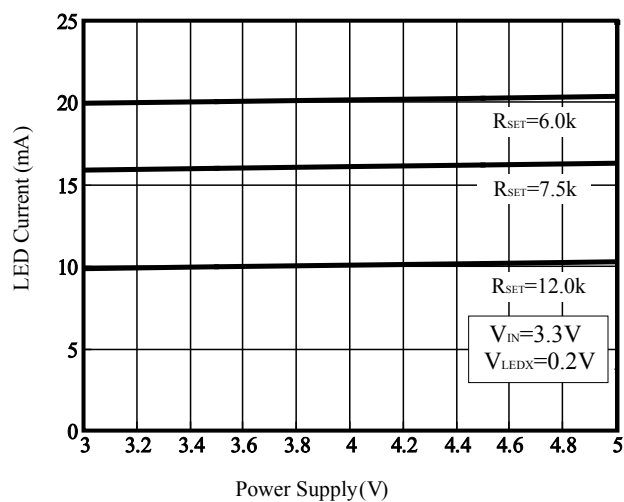
Figure 3 Power Supply vs. LED Current
