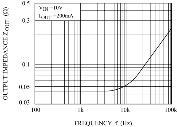
Z_{OUT} - f
