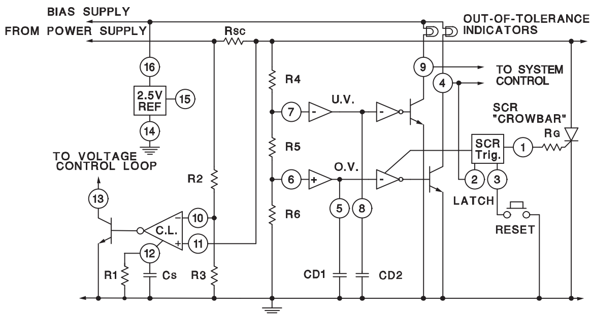
Figure 7. Typical Application
