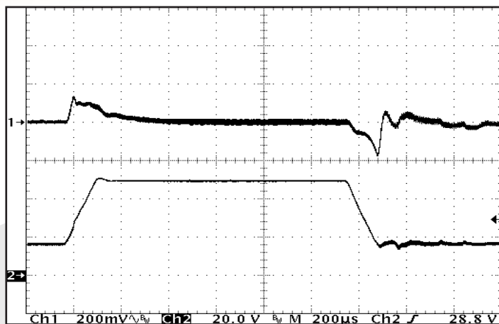
Figure 13: Output voltage response to step-change in input voltage (16 V - 50 V - 16 V). Load cap: 10 \mu F, 100m \Omega ESR tantalum cap and 1 \mu F ceramic cap. Ch 1: Vout (200 mV/div). Ch 2: Vin (20 V/div).
