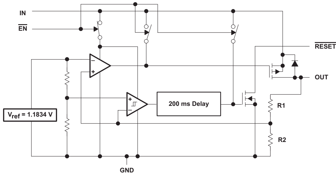
Figure 27. Fixed-Voltage Version
