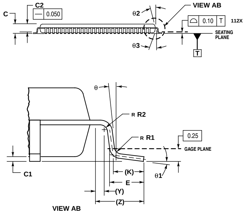
Figure B-2. 112-Pin LQFP Mechanical Dimensions (Case No. 987)
