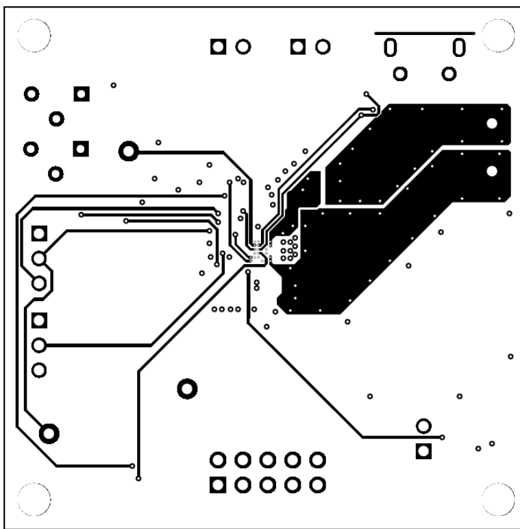
Figure 15. bq51221EVM-520 Layer 3
