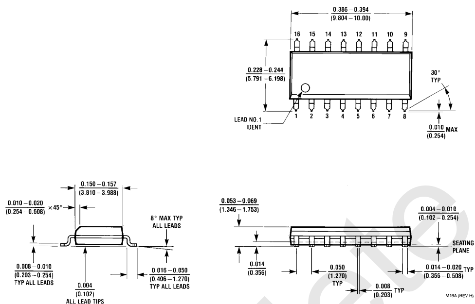
16-Lead Small Outline Molded Package (M) Order Number DM74LS174M or DM74LS175M NS Package Number M16A
