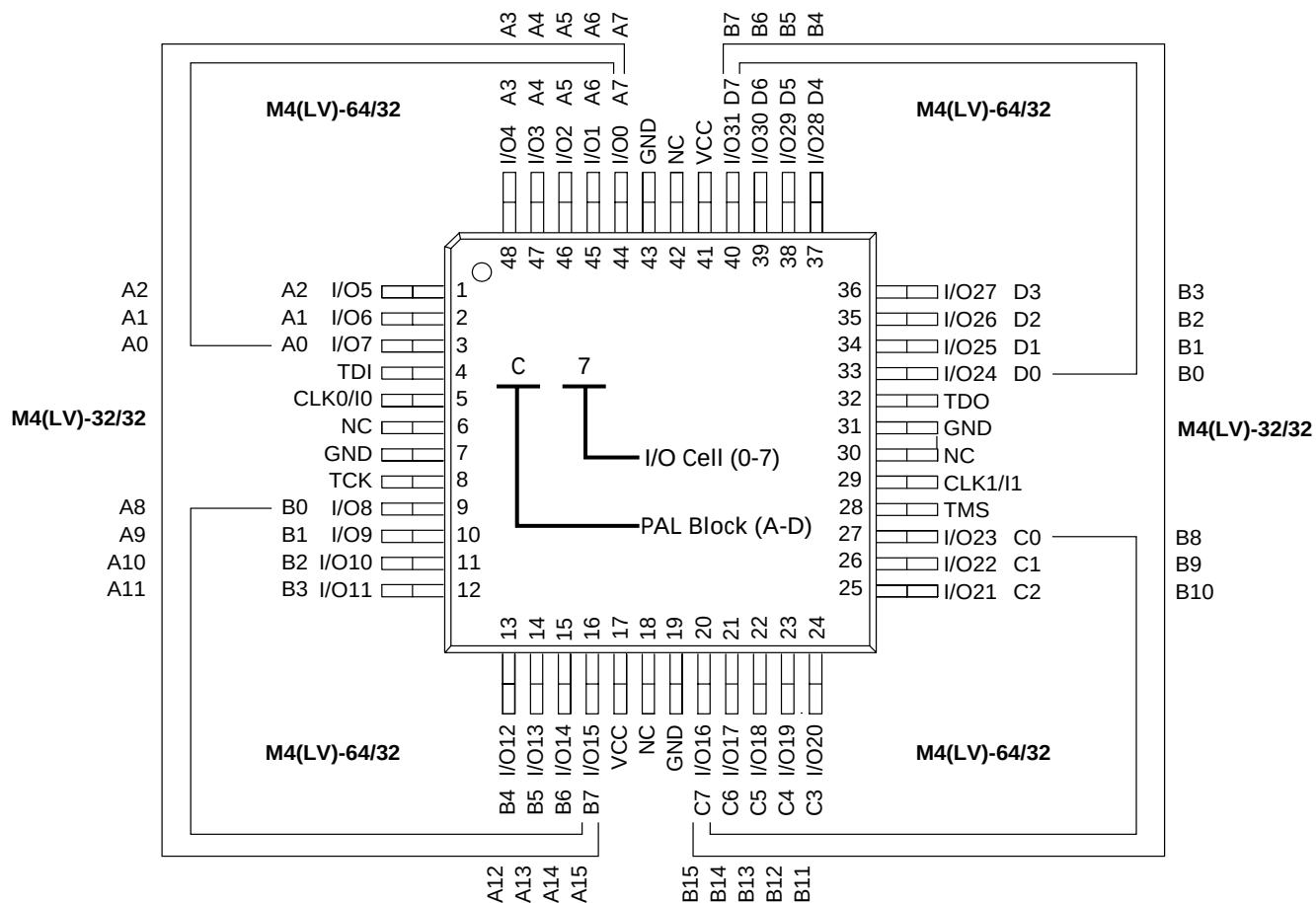
48-Pin TQFP
