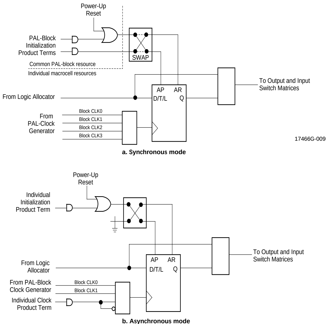
Figure 5. Macrocell
