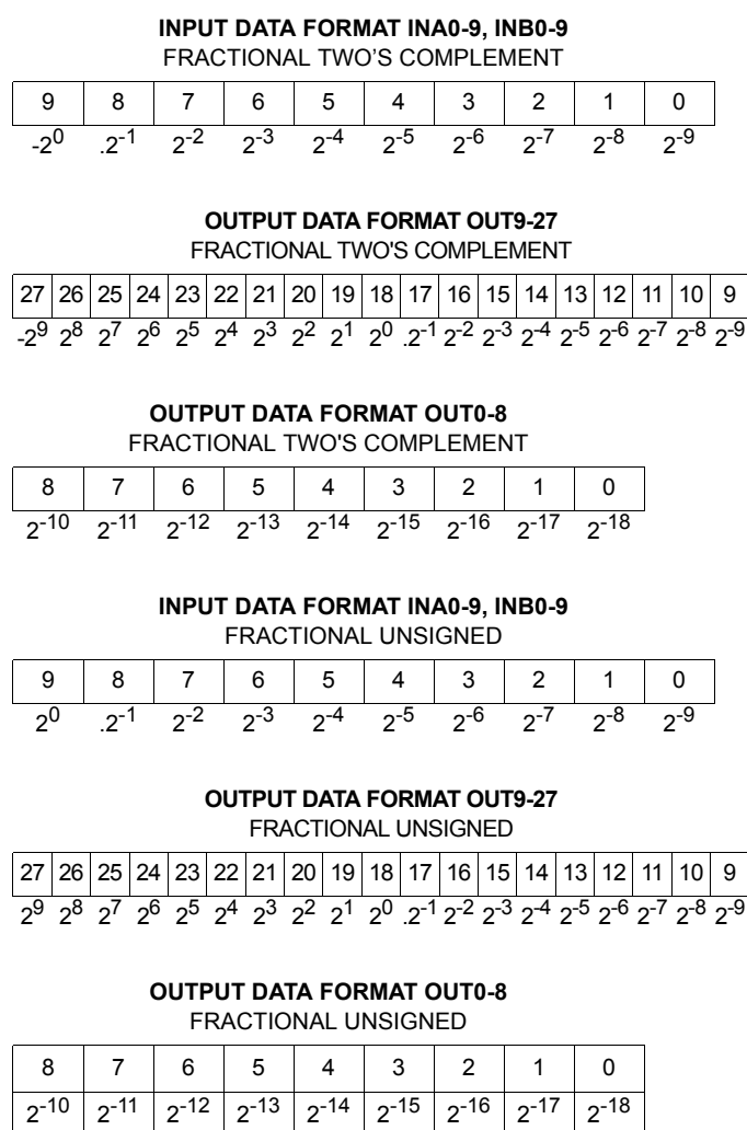
FIGURE 3. INPUT/OUTPUT FORMAT DEFINITIONS
