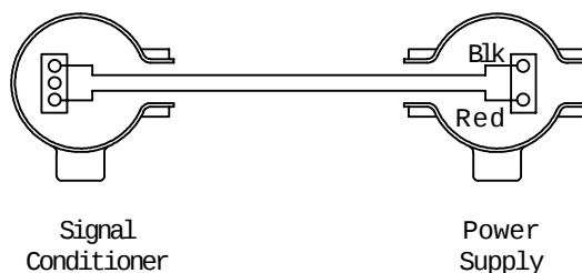
Power Supply to Signal Conditioner
