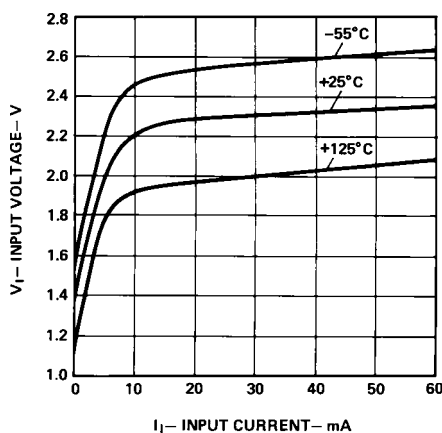
Figure 2. Input Characteristics.
