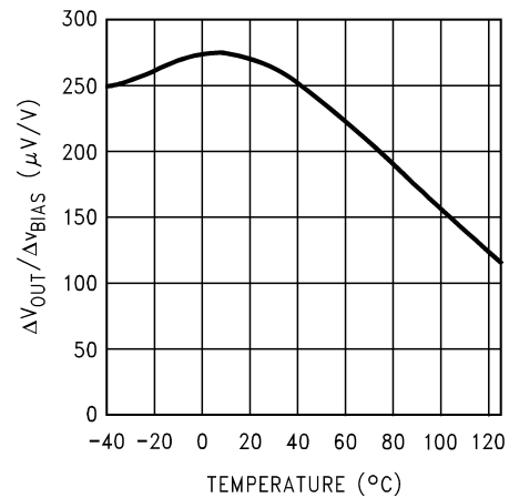
Line Regulation vs V_{BIAS}
