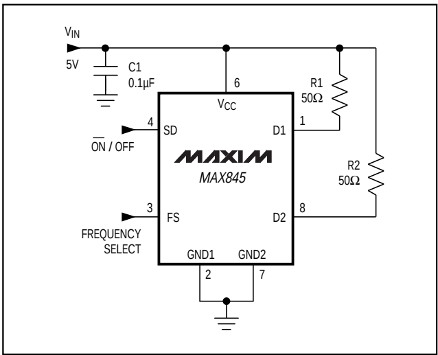
Figure 1. Test Circuit
