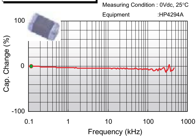
Murata MLCC 2220/47uF/16V
