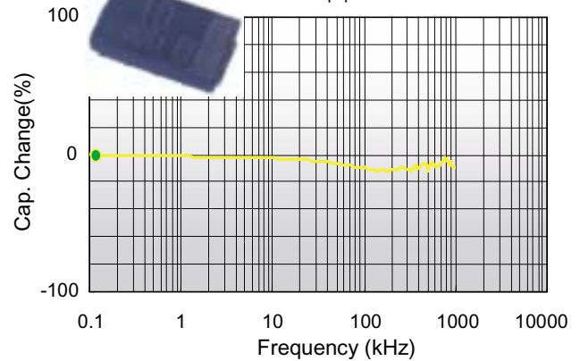
Organic 2918/10uF/10V
