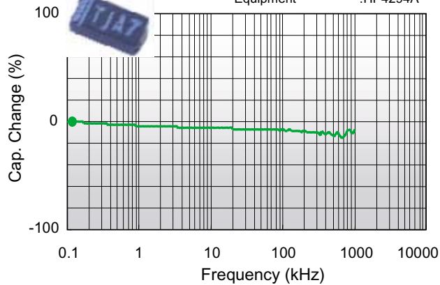
TA (X) 1206/10uF/6.3V
