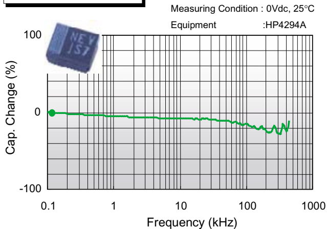
TA (X) 1411/47uF/6.3V
