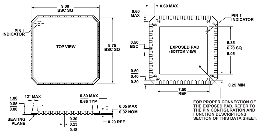
Figure 74. 64-Lead Lead Frame Chip Scale Package [LFCSP_VQ] 9 mm × 9 mm Body, Very Thin Quad CP-64-4
