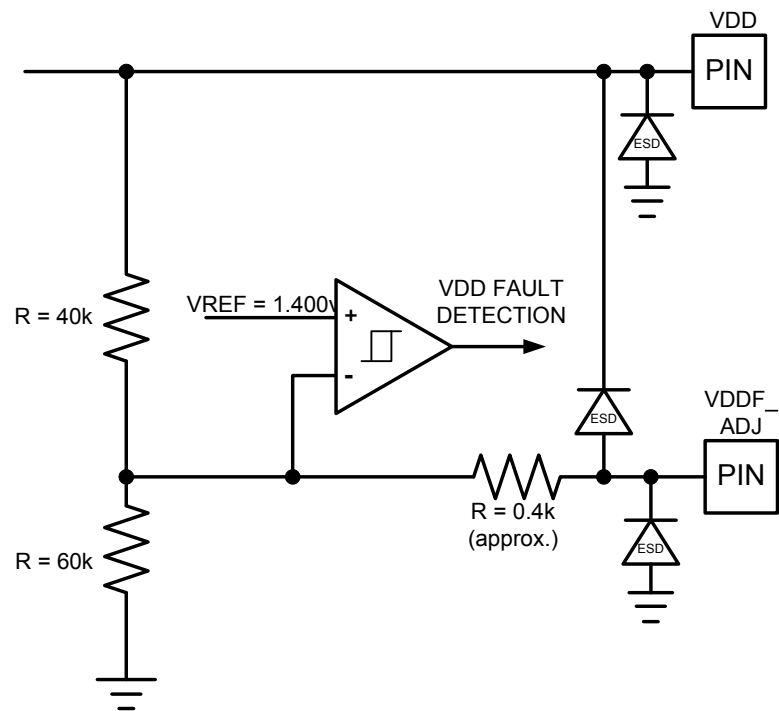
Figure 18: VDDF_ADJ
