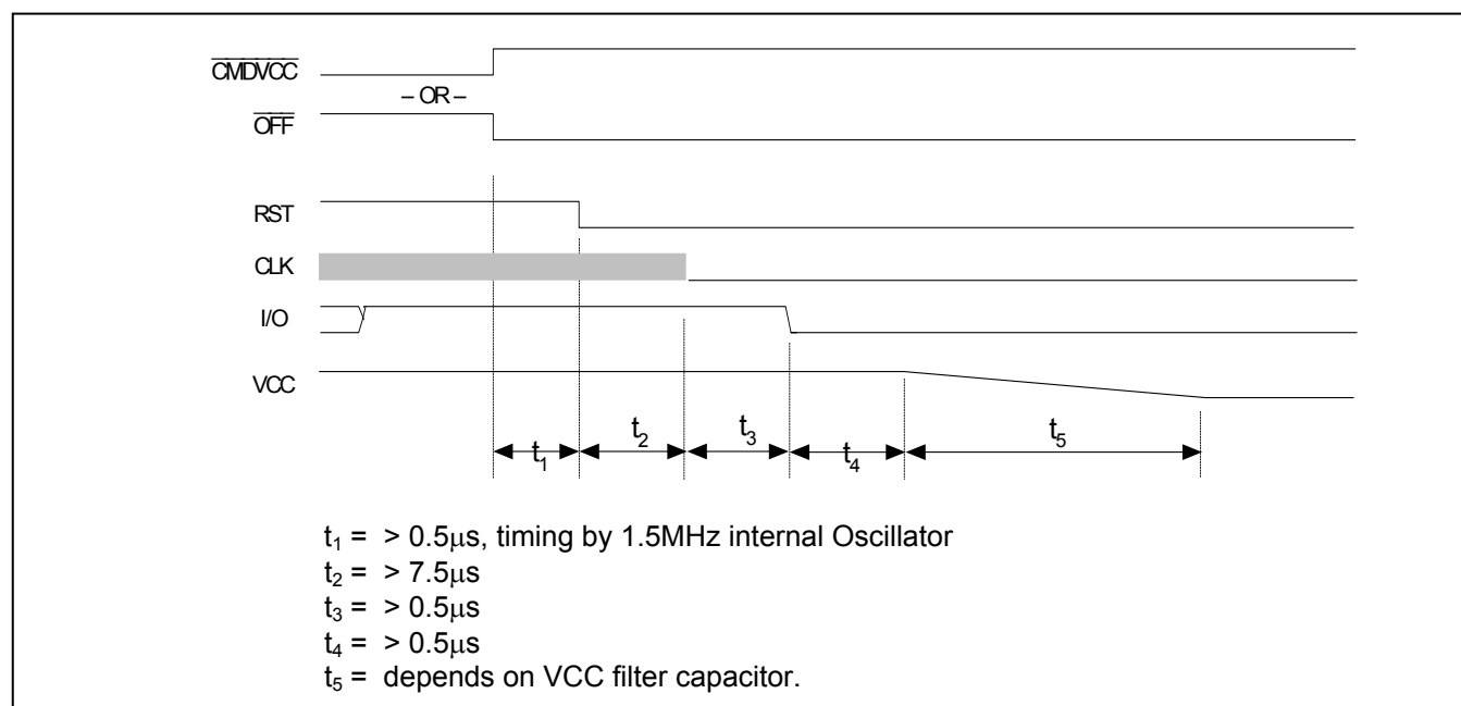
Figure 6: Deactivation Sequence
