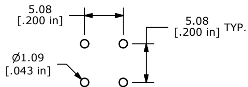
P.C. MOUNTING
