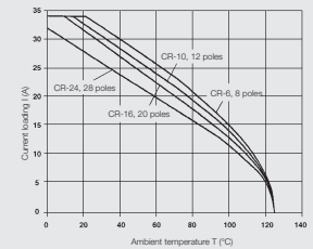
ConCept module CM-HE Conductor H07V-K 4.0 mm 2
