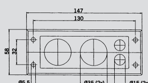
Cut-out size 24 35 x 117 mm
