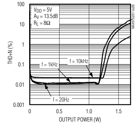
TOTAL HARMONIC DISTORTION PLUS NOISE vs. OUTPUT POWER (SPEAKER MODE)
