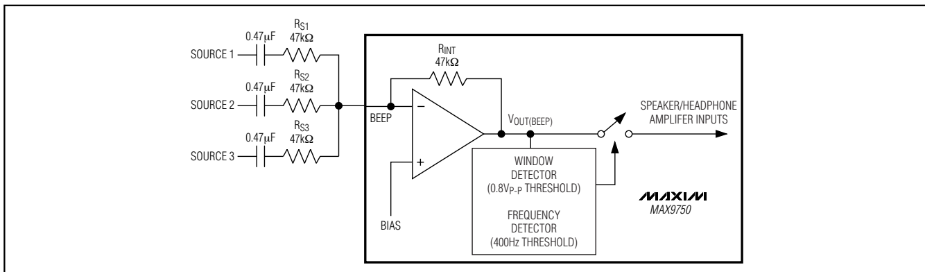
Figure 8. Beep Input
