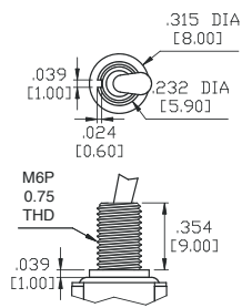
B8 Metric
