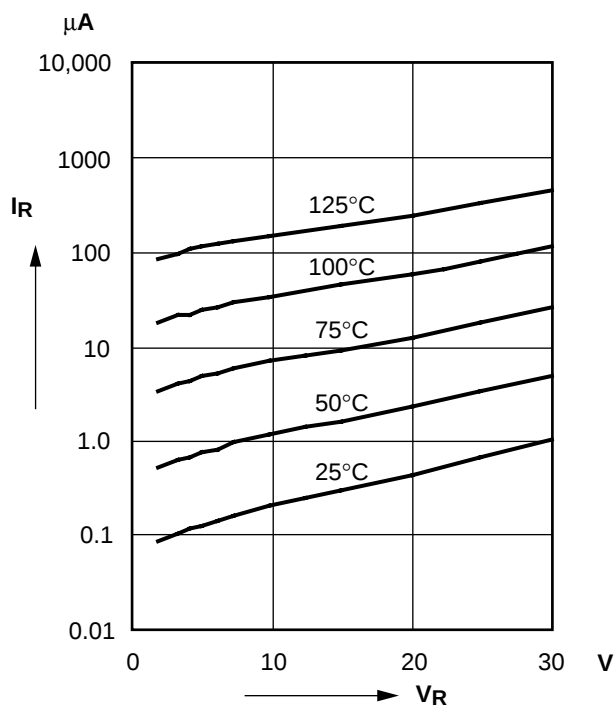
Typical variation of reverse current at various temperature
