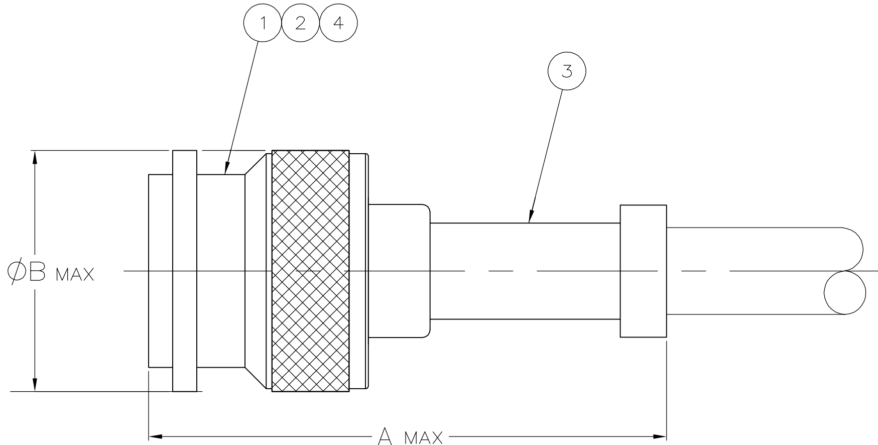
VIEW X
