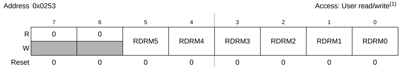
Figure 2-33. Port M Reduced Drive Register (RDRM)
