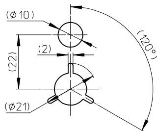
DETAIL "E"
