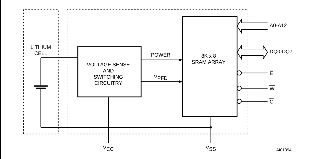
Figure 6. Block Diagram
