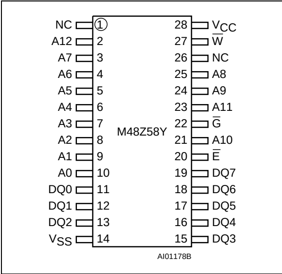
Figure 5. SOIC Connections
