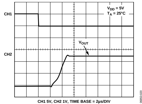
Figure 21. Exiting Power-Down Mode
