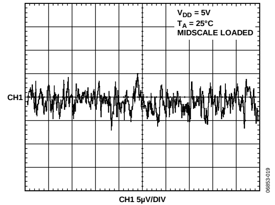
Figure 20. 1/f Noise, 0.1 Hz to 10 Hz Bandwidth
