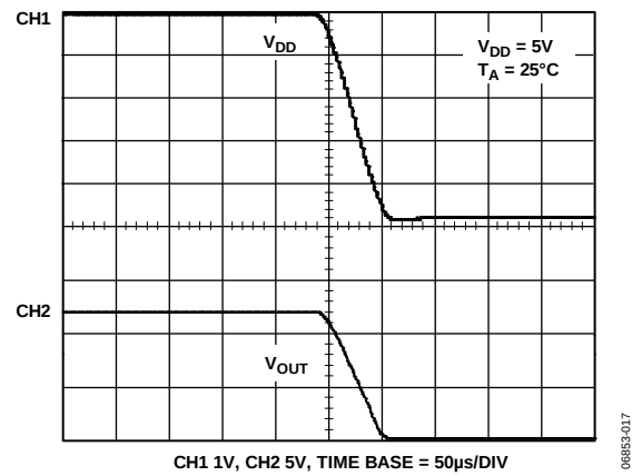
Figure 18. V_{DD} vs. V_{OUT}
