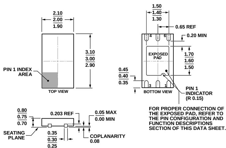
Figure 55. 6-Lead Lead Frame Chip Scale Package [LF CSP_WD] 2.00 x 3.00 mm Body, Very Very Thin, Dual Lead (CP-6-5)
