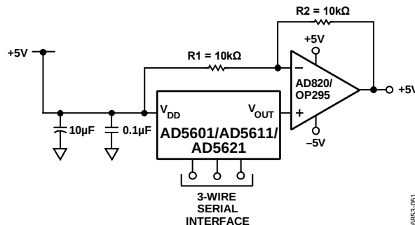
Figure 52. Bipolar Operation with the AD5601/AD5611/AD5621
