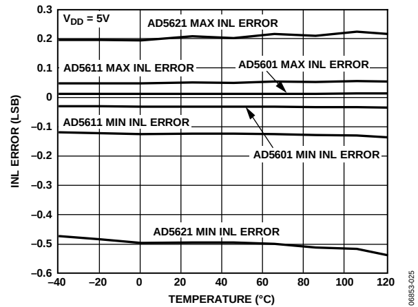
Figure 26. INL vs. Temperature (5 V)
