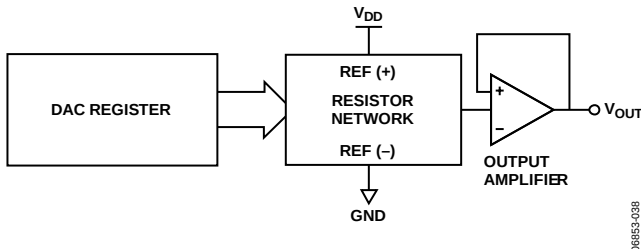
Figure 39. DAC Architecture
