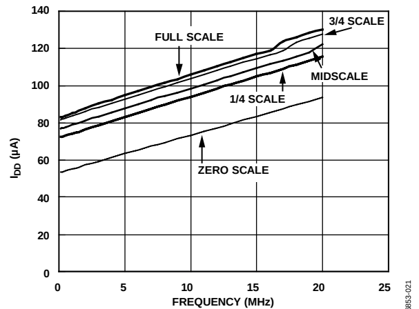
Figure 22. I_{DD} vs. SCLK vs. Code
