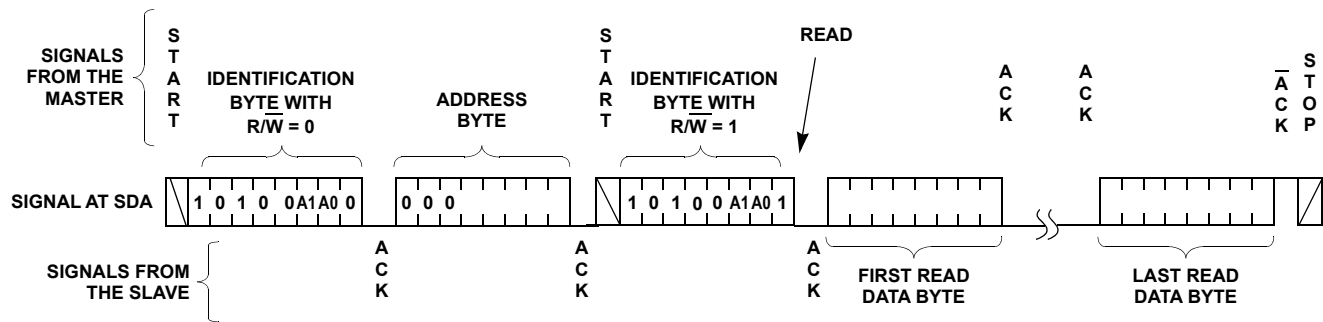
FIGURE 23. READ SEQUENCE
