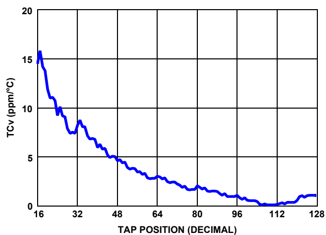
FIGURE 8. 100k TCv vs TAP POSITION
