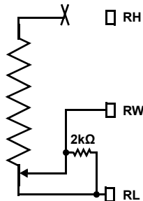
FIGURE 18. DCP CONNECTION IN SHUTDOWN MODE
