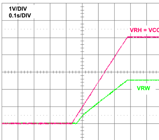
FIGURE 15. POWER-ON START-UP IN VOLTAGE DIVIDER MODE
