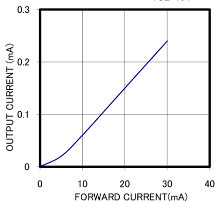
I_F VS I_o V_{CE} = 10\text{V}
