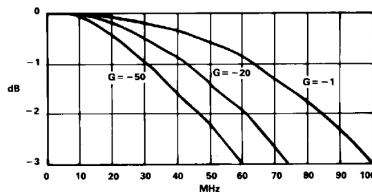
AD9610 Inverting Gain
