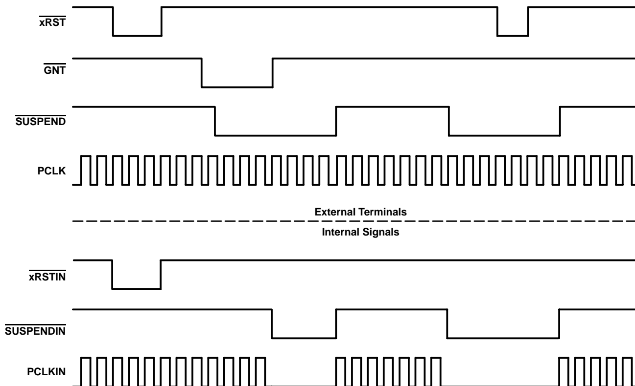
Figure 3–18. Signal Diagram of Suspend Function
