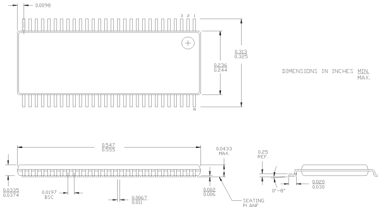
56-Lead Thin Shrunk Small Outline Package Z56
