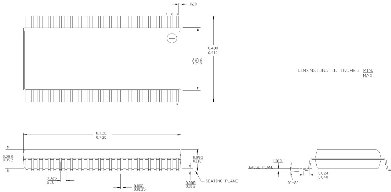
56-Lead Shrunk Small Outline Package Q56
