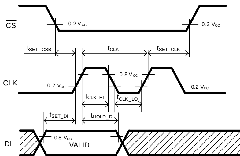
Figure 6. SPI Timing
