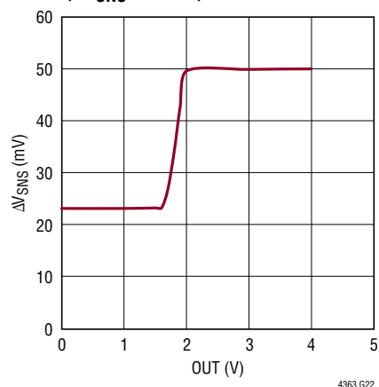
Current Limit Foldback ( \Delta V_{SNS} vs OUT )
