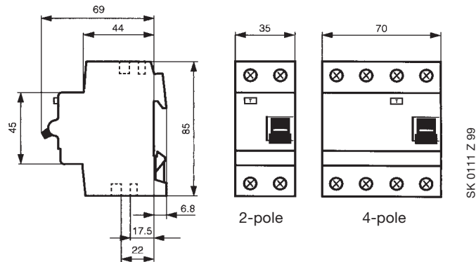
F 202, F 204, F 204 S
