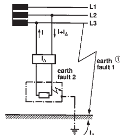
IT system
