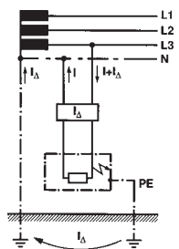
TT system
