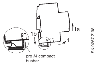
B Detaching when pro M compact cross wiring remains in place
