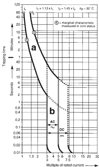
trip characteristic: B I_n = 6 \dots 63 \text{ A} S 200/S 200 M MCBs
