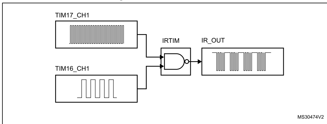
Figure 5. Infrared transmitter
