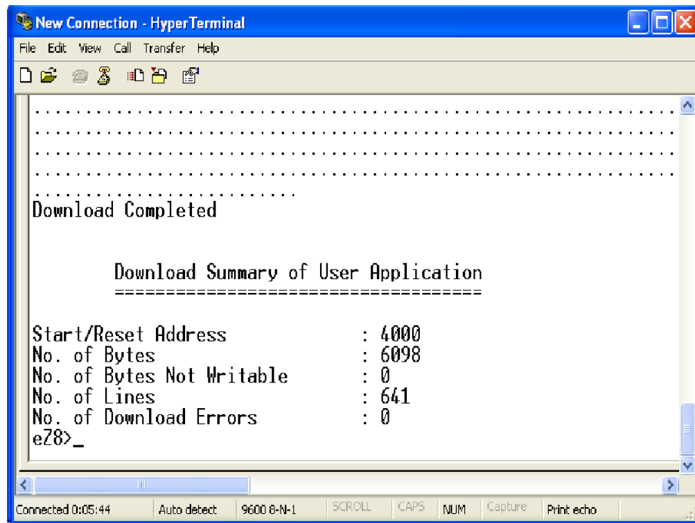
Figure 8. Flash Loader Screen Displays HEX File Download Completion Summary
