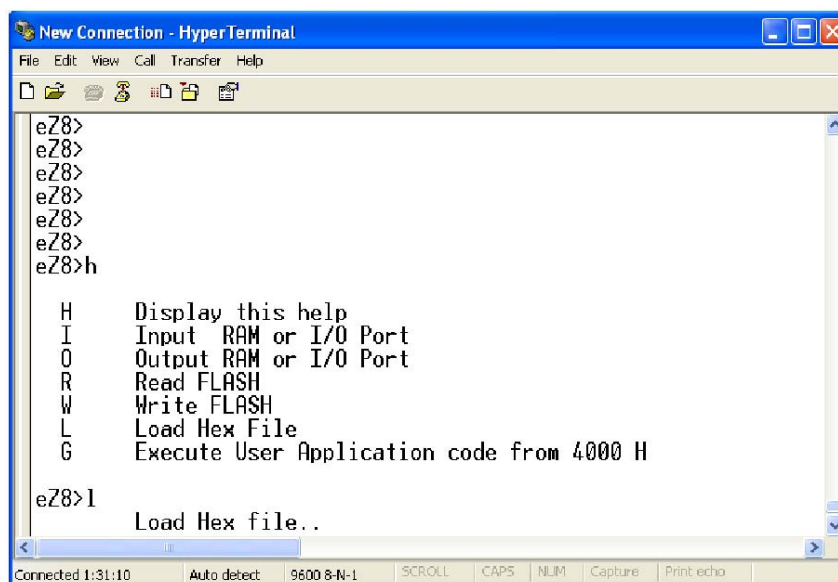
Figure 6. Flash Loader Screen Displays Start of HEX File Download
