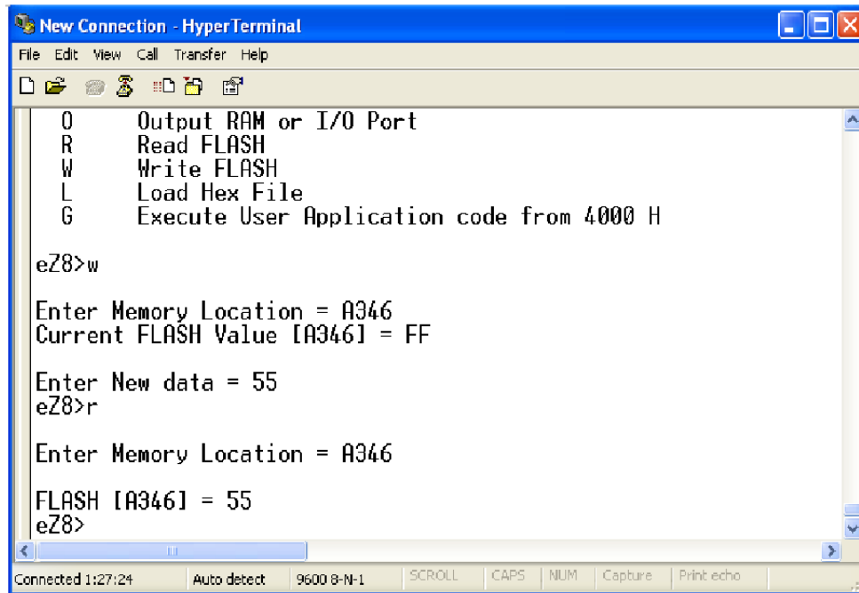
Figure 5. Flash Loader Screen Displays Flash Write Capability
