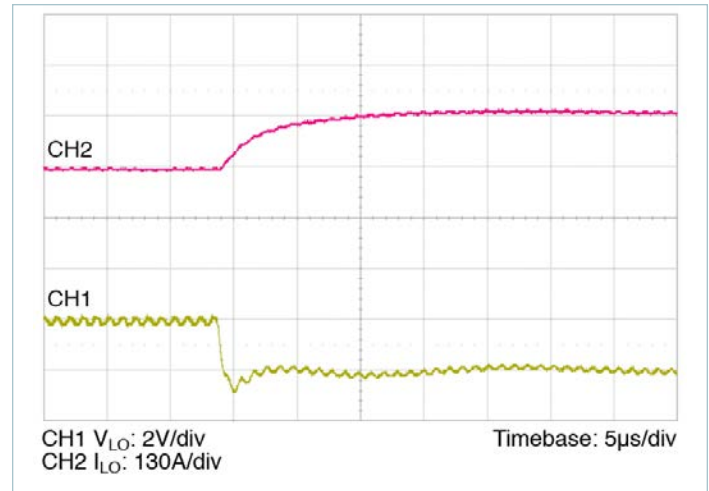
Figure 15 — 0A – 130A transient response: C_{HI\_IN\_EXT} = 300\mu F , no external C_{LO\_OUT\_EXT}
