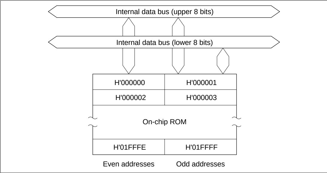
Figure 18.28 ROM Block Diagram (H8/3067)
