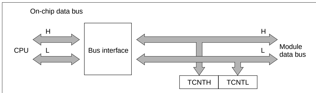
Figure 9.4 Access to Timer Counter (CPU Writes to TCNT, Word)
