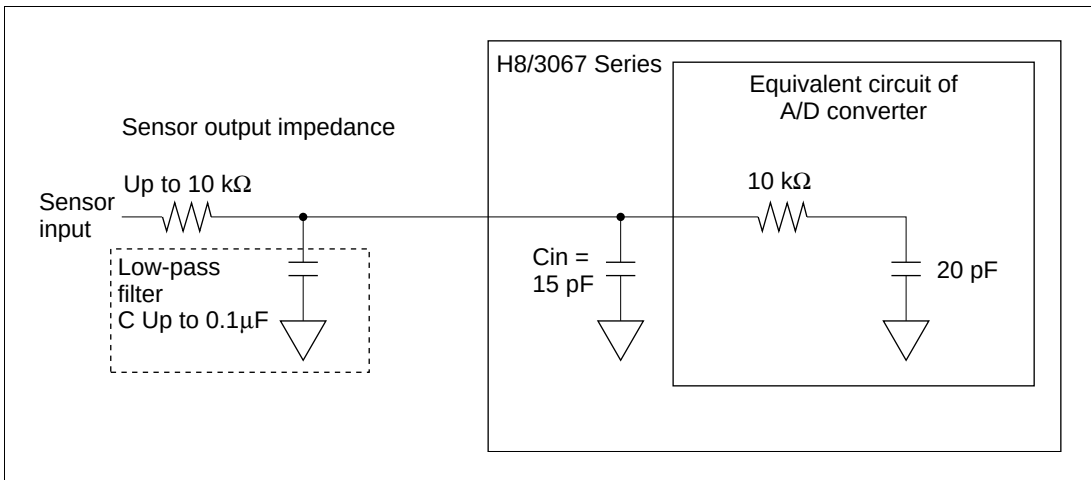
Figure 15.11 Analog Input Circuit (Example)
