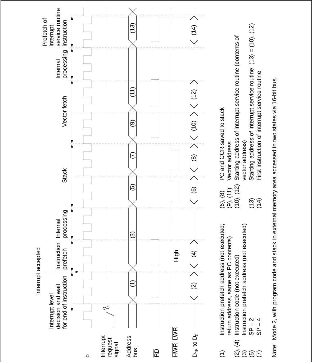
Figure 5.7 Interrupt Sequence
