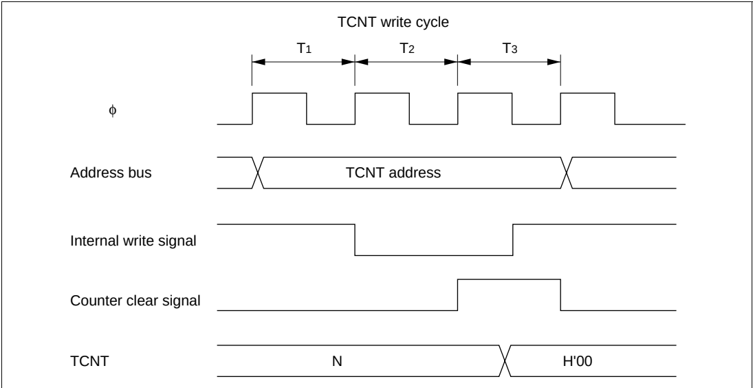
Figure 10.18 Contention between TCNT Write and Clear
