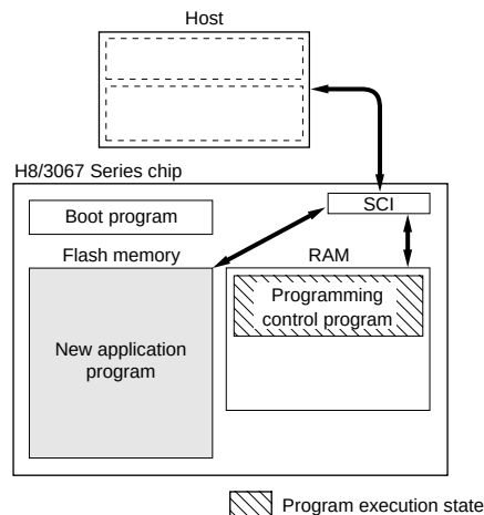
Figure 18.3 Boot Mode
