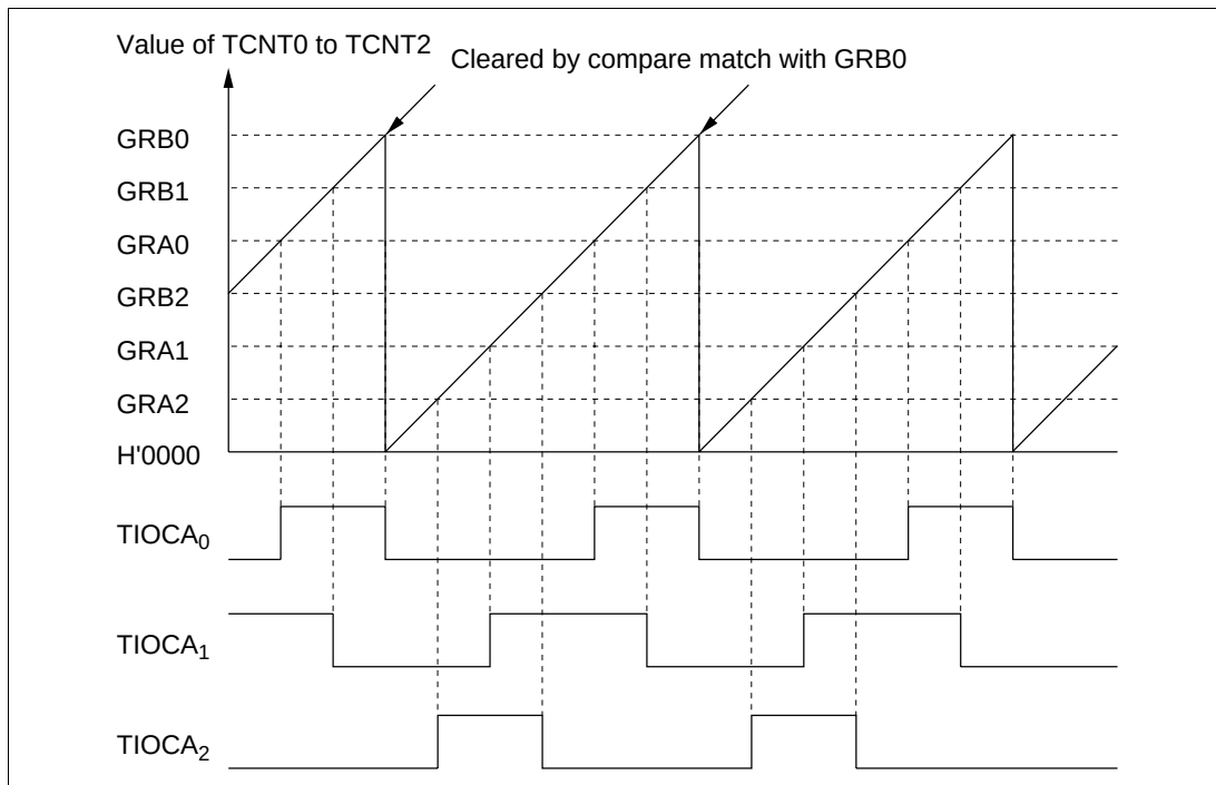
Figure 9.25 Synchronization (Example)
