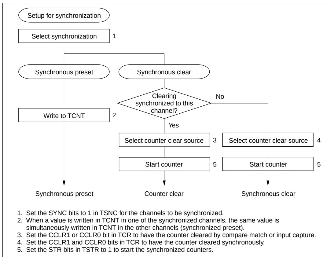
Figure 9.24 Setup Procedure for Synchronization (Example)
