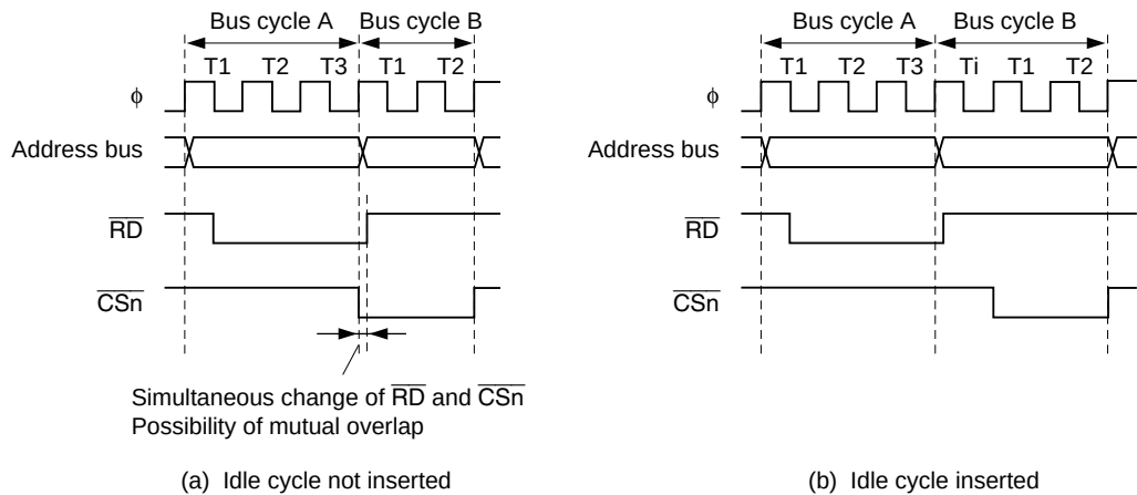
Figure 6.47 Example of Idle Cycle Operation (5)
