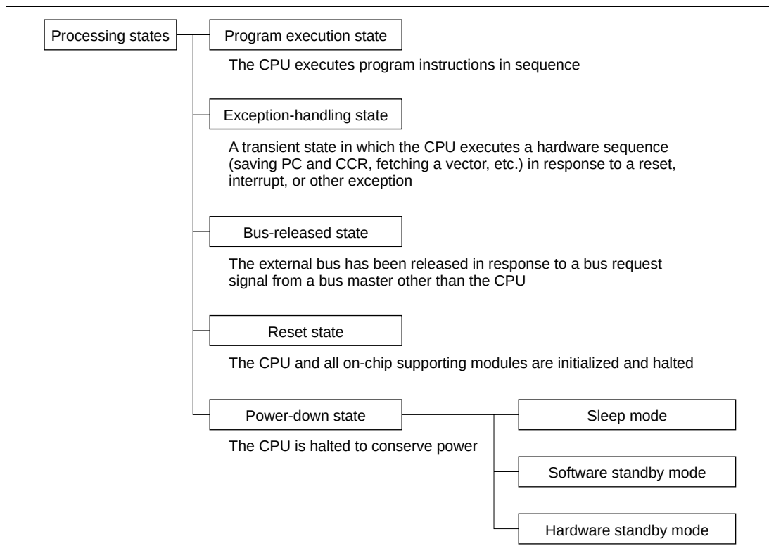
Figure 2.11 Processing States
