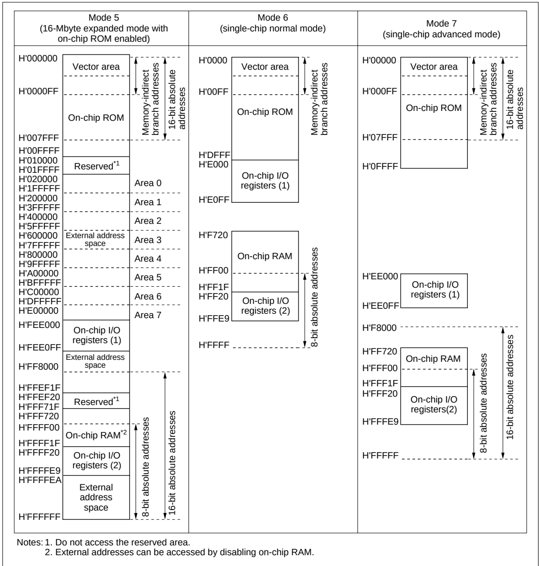
Figure 3.3 H8/3065 Memory Map in Each Operating Mode (2)
