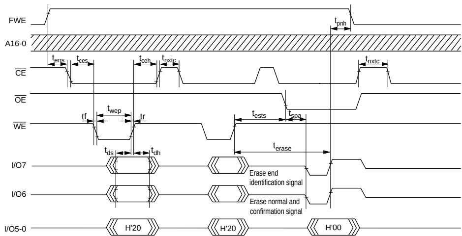
Figure 18.21 Auto-Erase Mode Timing Waveforms
