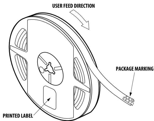
Figure 16 Reeling Orientation
