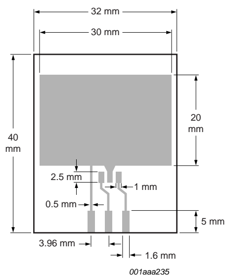
Fig.16 FR4, mounting pad for collector 6 cm 2 .
