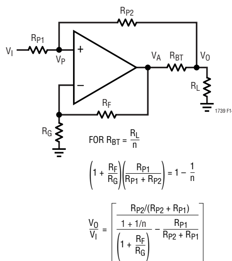
Figure 14. Back Termination Using Positive Feedback
