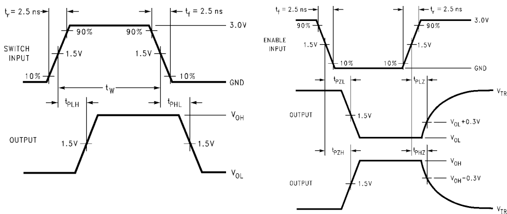
FIGURE 2. AC Waveforms
