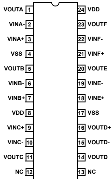
EL5611 (24-PIN HTSSOP) TOP VIEW
