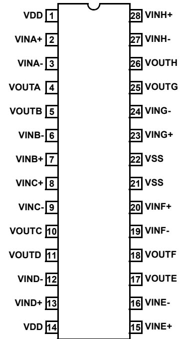
EL5811 (28-PIN HTSSOP) TOP VIEW
