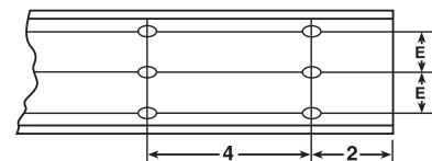
Bottom Mounting Holes, 1/2 x 3/16
