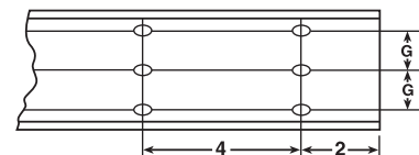
Bottom Mounting Holes, 1/2 x 3/16
