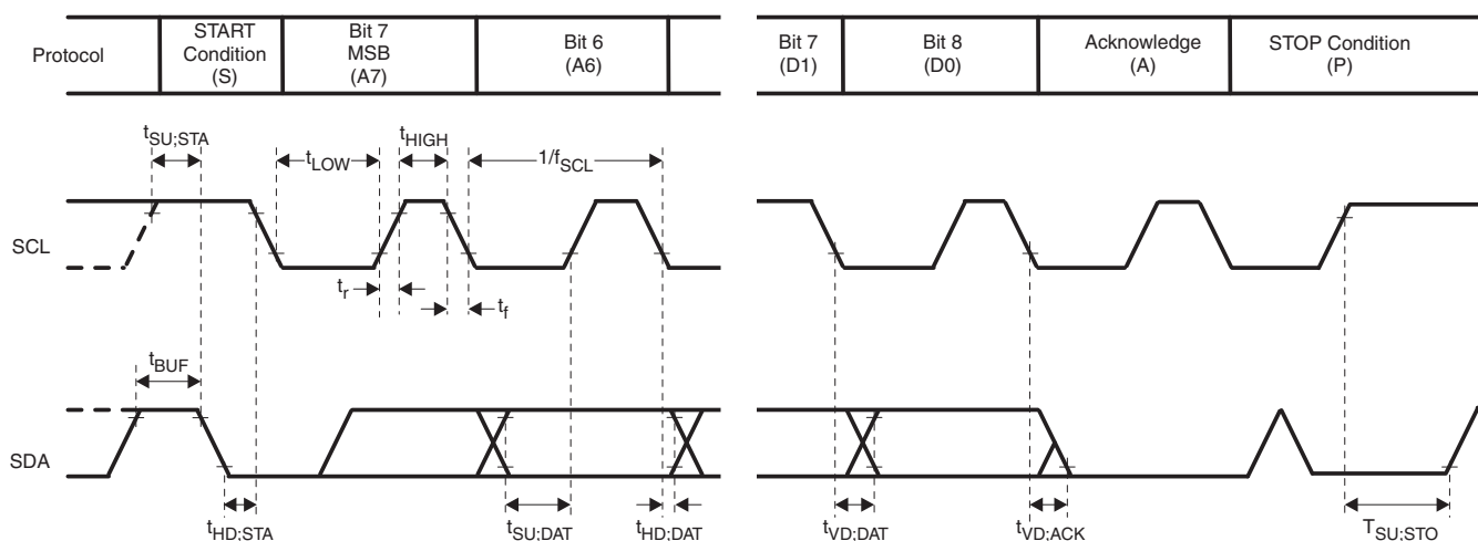
Figure 3. I²C Bus Timing
