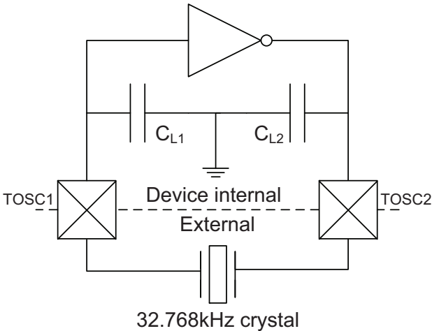
Figure 33-11.TOSC input capacitance.
