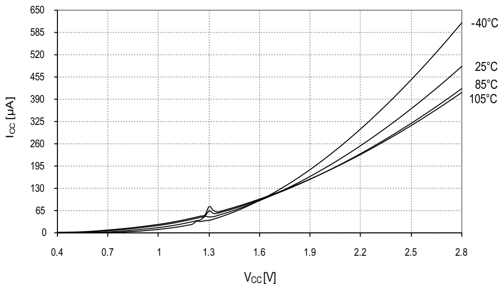
Figure 34-143. Power-on reset current consumption vs. V_{CC} . BOD level = 3.0V, enabled in sampled mode.
