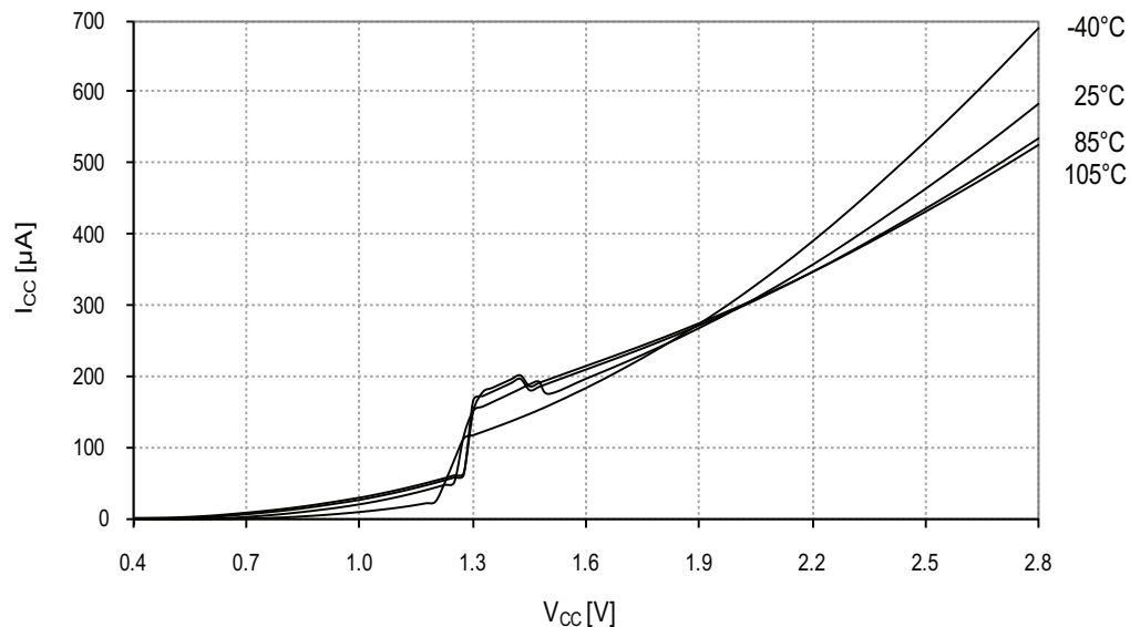
Figure 34-142. Power-on reset current consumption vs. V_{CC} . BOD level = 3.0V, enabled in continuous mode.
