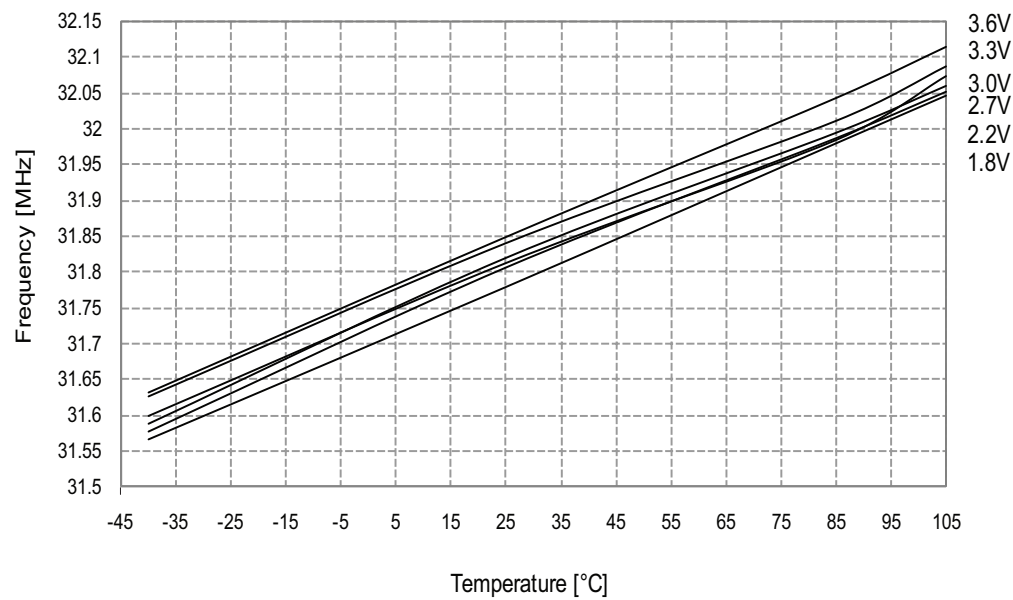
Figure 34-72. 32MHz internal oscillator frequency vs. temperature. DFLL enabled, from the 32.768kHz internal oscillator.
