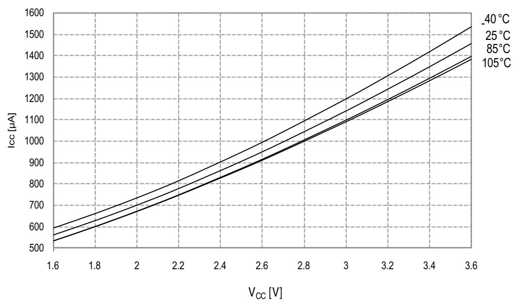
Figure 34-93. Idle mode current vs. V_{CC} .
