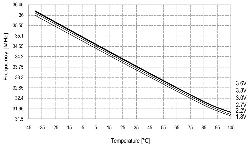
Figure 34-72. 32MHz internal oscillator frequency vs. temperature. DFLL enabled, from the 32.768kHz internal oscillator.
