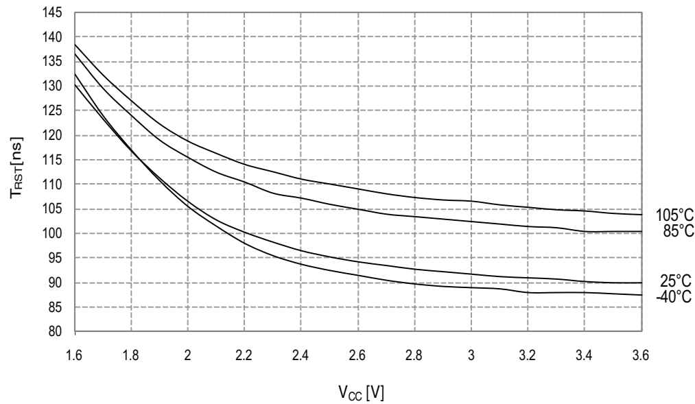
Figure 34-57. Minimum Reset pin pulse width vs. V_{CC} .
