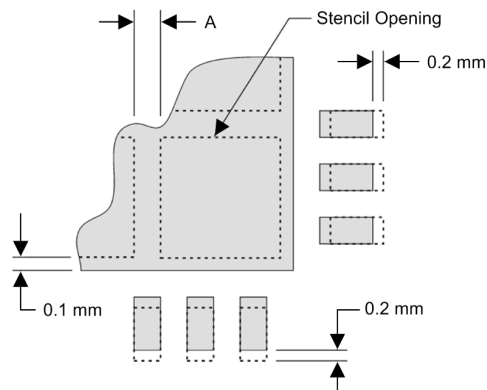
Figure 39. No Pullback LLP, Single Row Reference Diagram
