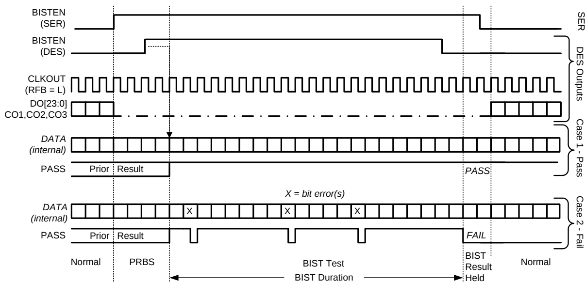
Figure 29. BIST Waveforms
