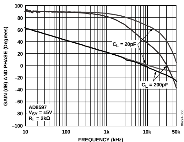
Figure 30. Gain and Phase vs. Frequency
